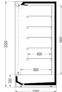
Mendos LU.SP/EP-A L
