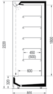
Mendos EU.SP/EP-A L
